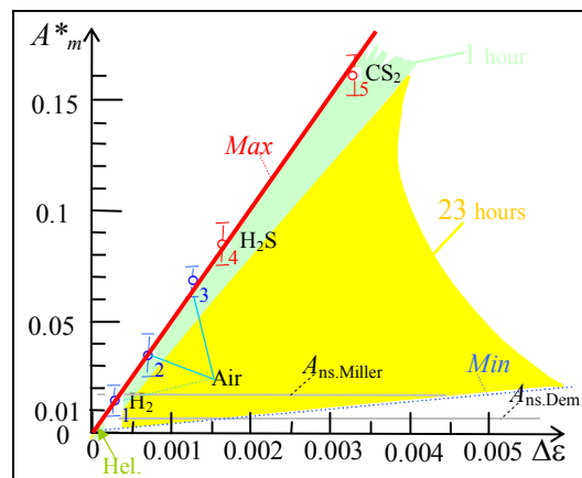
Fig.1. The dependence of the A_m(\Delta\varepsilon) amplitude A_m of the interference fringe shift from the polarization contribution \Delta\varepsilon_{\text{ptcl.}} particles to the total permittivity \varepsilon=1+\Delta\varepsilon_{\text{ptcl.}} light-carrying medium the Michelson interferometer (MI), discovered by me in 1968 (for l_{\parallel}=l_{\perp}=7 m, and \lambda=6\cdot 10^{-7} m) [3]:
